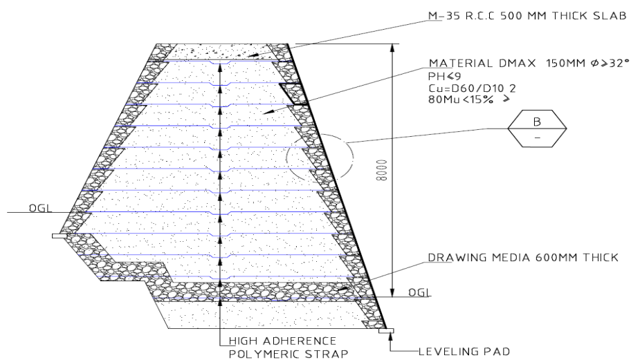
DEFLECTOR DAM
